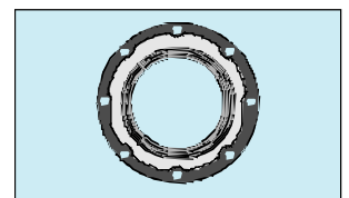
Multi-Class
